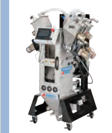
Gravimetric Batch Blender AUTOCOLOR II
